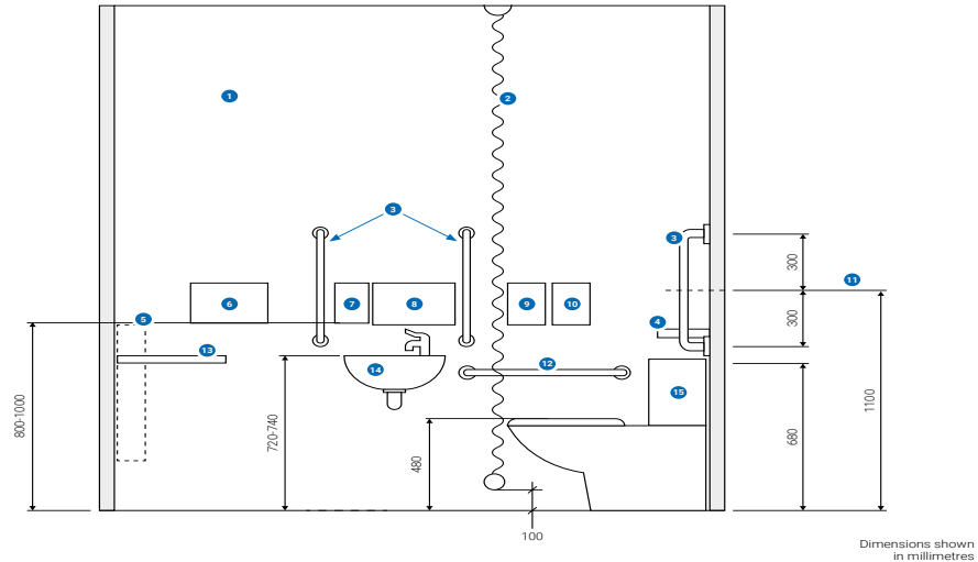
Doc M Installation – Side View
